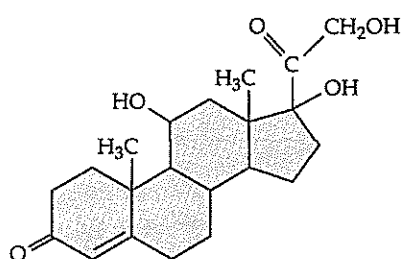
Cortisol molecule
